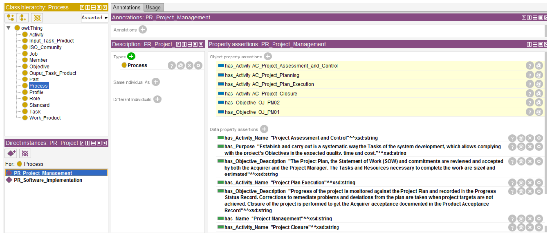
Figure 8. Inferences deduced by the reasoner Pellet shown in yellow for the individual PR_Project_Management in the Protégé framework
