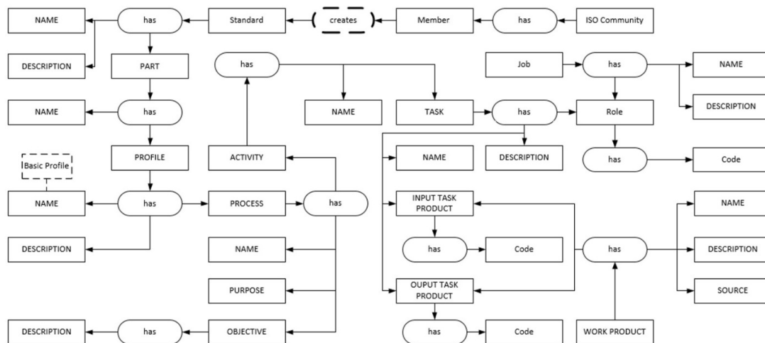
Figure 2. Executable pre-conceptual schema related to the Basic Profile of the ISO/IEC 29110
