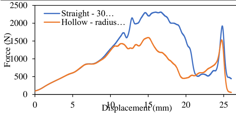
Figure 2. Numerical results of force vs. displacement of tested blades.
