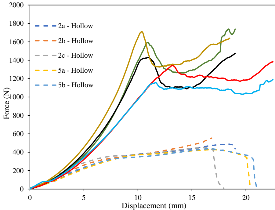
Figure 9. Experimental results of the cutting tests in only rubber samples for straight (solid line) and hollow blades (dashed lines).
