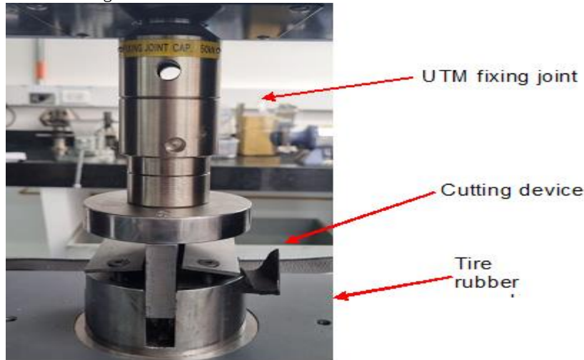
Figure 6. Built cutting device mounted on the UTM.
