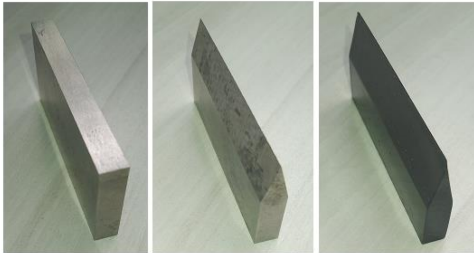
Figure 4. Manufactured blades. (a) 90° profile (b) 30° straight profile (c) hollow profile.
