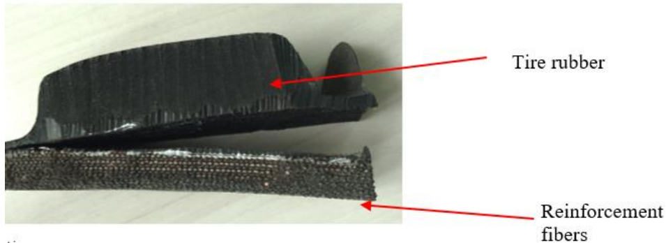
Figure 8. Separated rubber from reinforcement fibers of a section of a used tire band.
