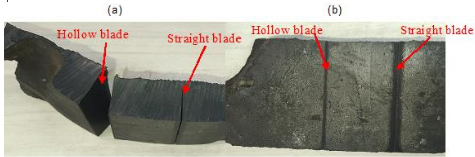
Figure 10. Remaining marks on the rubber samples after the cutting tests. (a) Side view, (b) Top view.
