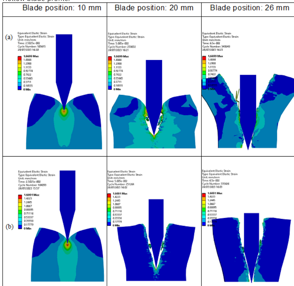
Figure 3. Evolution of the cutting process of tire rubber for (a) straight 30° blade profile, (b) Hollow blade profile.
