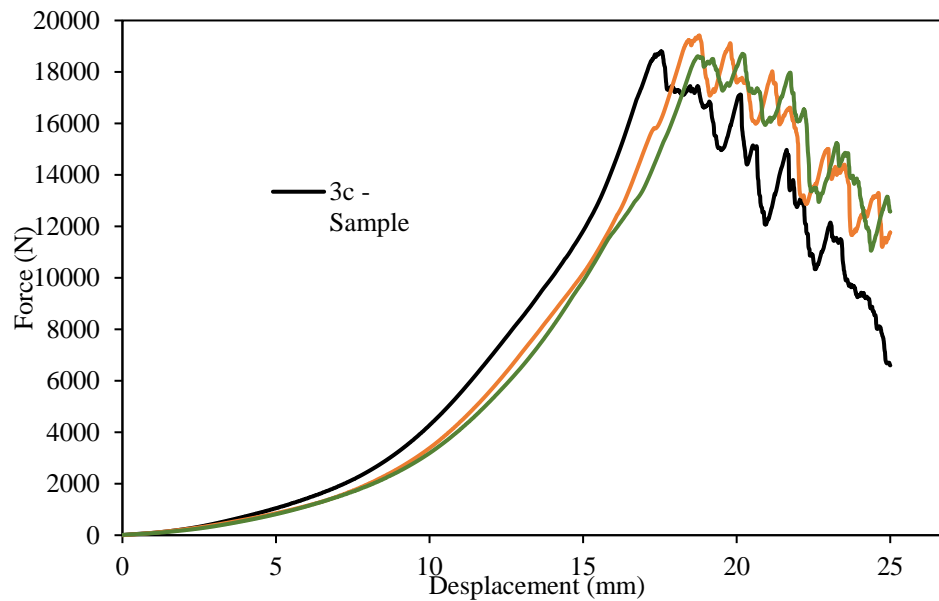
Figure 12. Experimental results of the cutting tests with the 90° straight profile. Source: own elaboration.
