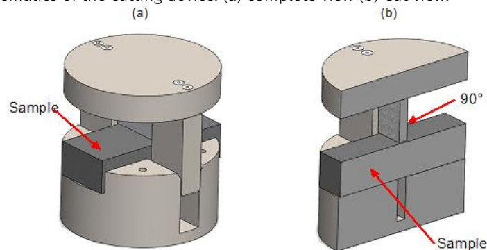
Figure 5. Schematics of the cutting device. (a) complete view (b) Cut view.
